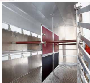
TA510G 12'x5'10"x7' High Headroom Horse & Livestock Trailer Available with or without Fold-up Sheep Deck. (Centre horse partition optional extra).
