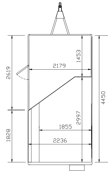
Trailer with no accommodation fit-out
